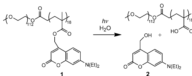
Scheme 1. Chemical structure and photolysis of the coumarin-containing amphiphilic block copolymer 1 .
